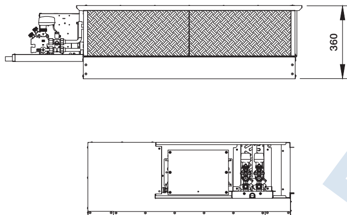
General Arrangement drawing
